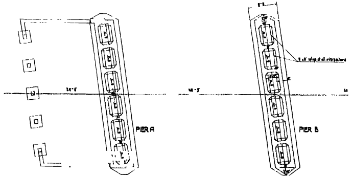
HALF SECTIONAL PLAN OF PIERS.
